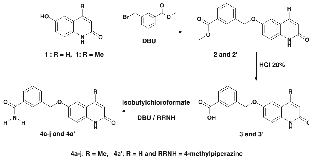
Scheme 1. General procedure for the synthesis of compounds 4a-j and 4a' .
